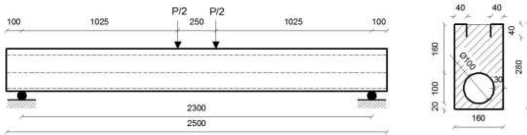
Figure 1. Dimensions and details of the specimen.
