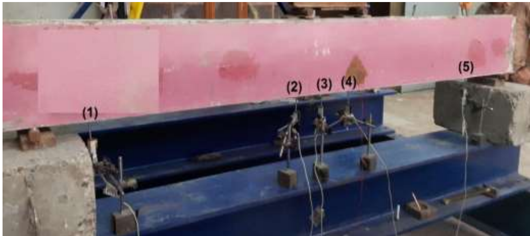
Figure. 5. LVDT locations.
