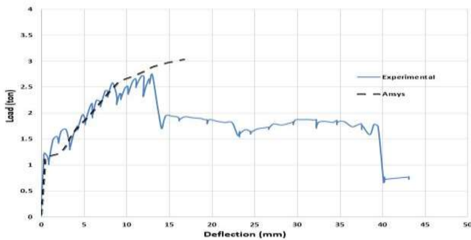
Figure 15. Comparison between experimental & numerical load-deflection curves of tested specimen (SIPU).
