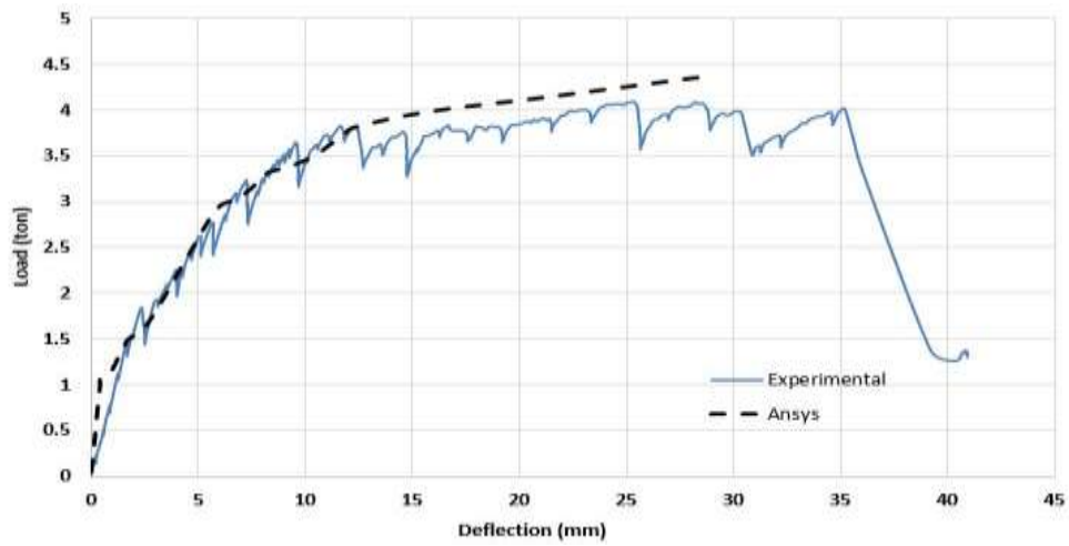
Figure. 16. Comparison between experimental & numerical load-deflection curves of tested specimen (SIPUR).
