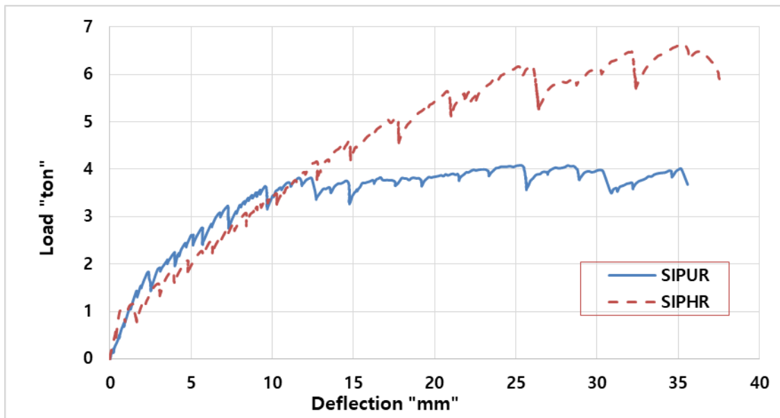
Figure. 10. Comparison between Load-Central deflection relationships of the specimens (SIPUR and SIPHR).
