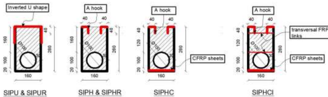
Figure 4. Shapes of the stay-in-place forms.
